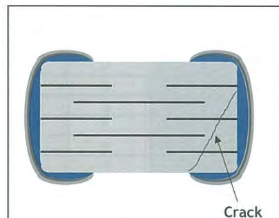
Fig. 7 Floating design (one kind of open-mode design) – circuit open during cracking.
