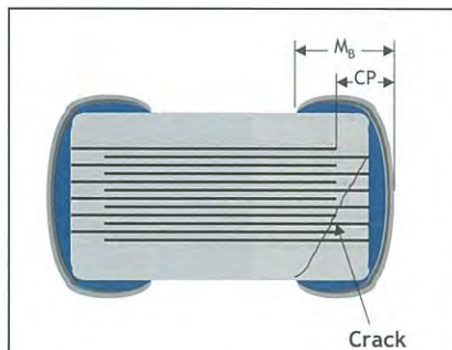
Fig. 5 Normal design (CP<Mb) – circuit leakage during cracking.
