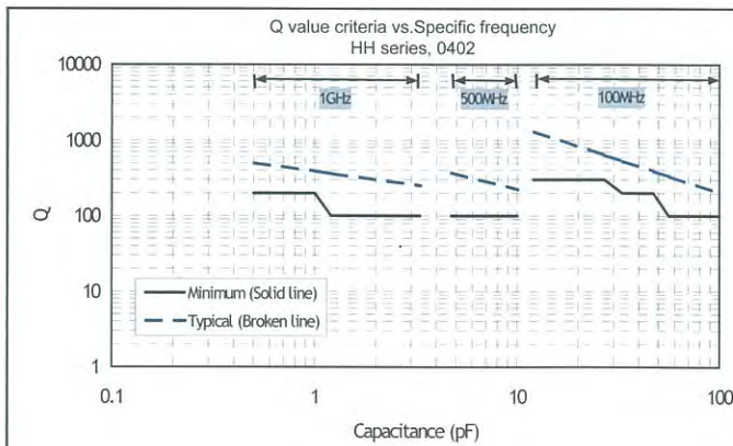
Fig. 1 Q factor specification vs. Specific frequency 0402
