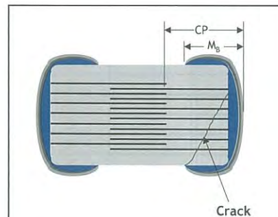
Fig. 6 Open-mode design (CP>Mb) – circuit open during cracking.
