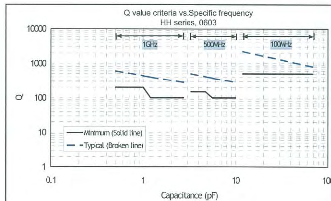
Fig. 2 Q factor specification vs. Specific frequency 0603
